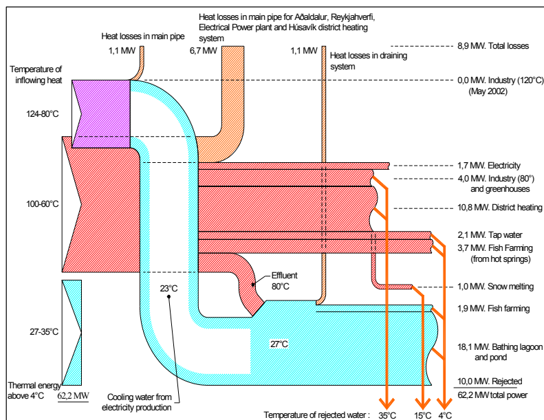
Fig 4.1 A flow chart depicting the utilization of thermal energy above 4°C at maximum load
