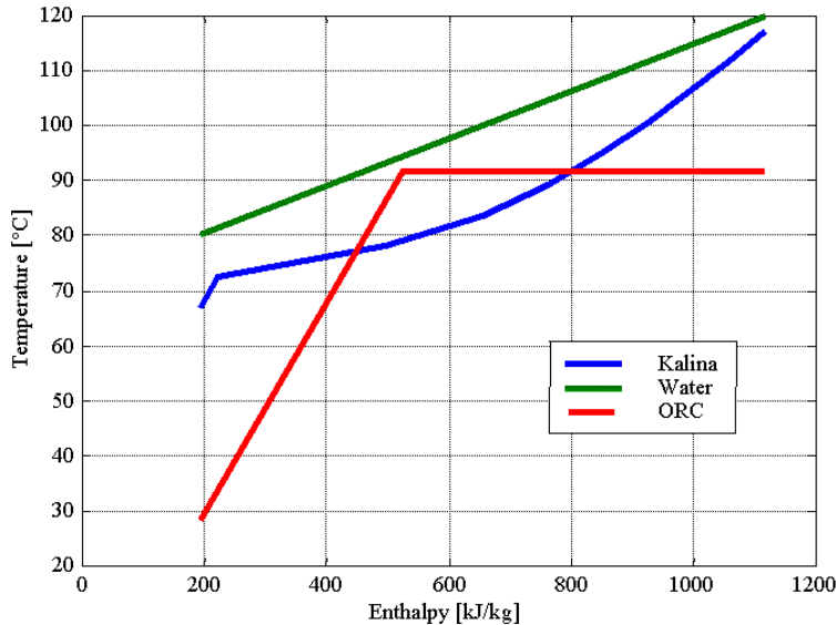
Fig 3.3.2. Comparison between boiling of the ammonia-mixture, pentane (ORC) and pure water.
