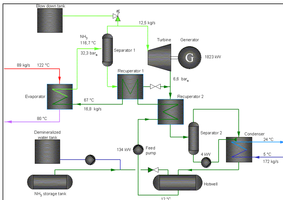
Fig 3.3.1 Power Plant – Schematic diagram
