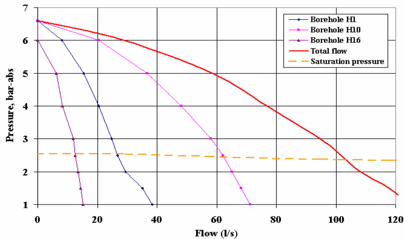
Fig 2.2. Hveravellir – Well performance.
