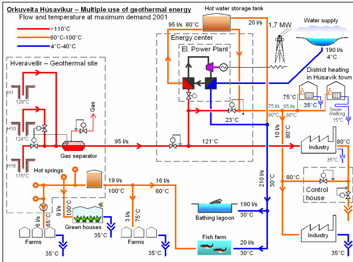
Fig. 3.2.1. Húsavík Energy – Multiple use of geothermal energy – Process diagram
